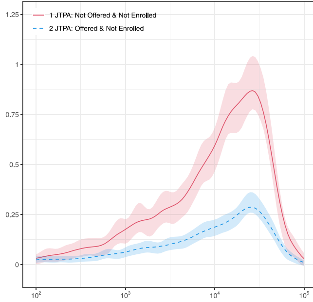
Fig. 3. Testing validity of instruments, JTPA. Notes: (i) JTPA: Not Offered & Not Enrolled: the scaled density estimate \frac{\sum_i 1(t_i=0, d_i=0)}{\sum_i 1(d_i=0)} \hat{f}_{d=0, t=0}(x) ; (ii) JTPA: Offered & Not Enrolled: the scaled density estimate \frac{\sum_i 1(t_i=0, d_i=1)}{\sum_i 1(d_i=1)} \hat{f}_{d=1, t=0}(x) . Point estimates are obtained by using local polynomial regression with order 2, and robust confidence bands are obtained with local polynomial of order 3. Bandwidths are chosen by minimizing integrated mean squared errors. All estimates are obtained using companion R (and Stata) package described in Cattaneo et al. (2021b).
