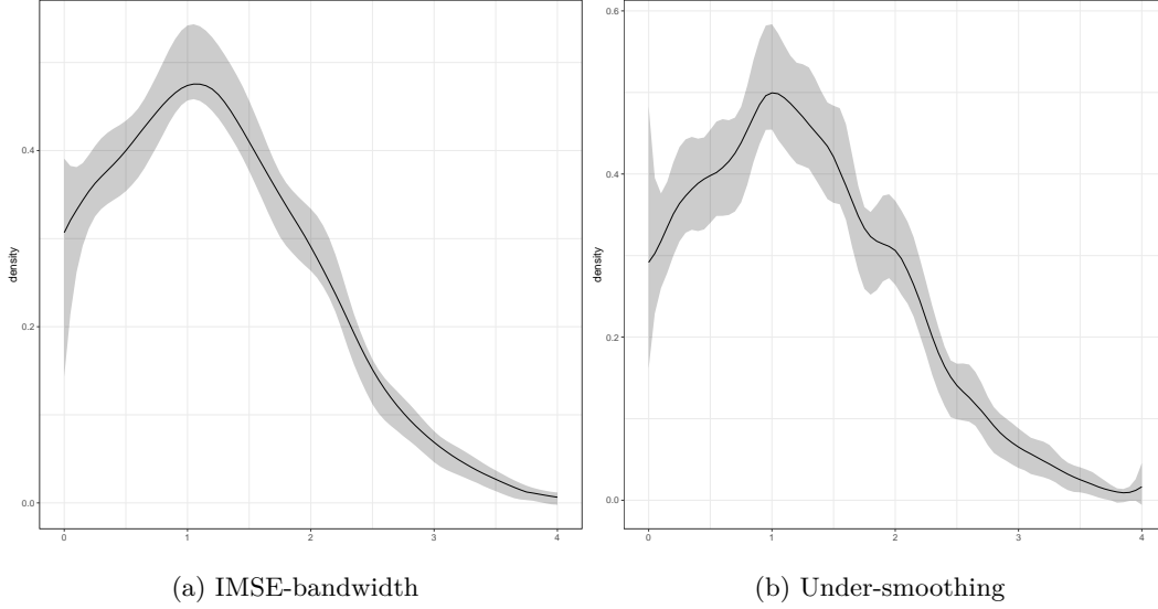
Figure 3: Density plot with IMSE-optimal bandwidth and under-smoothing.
