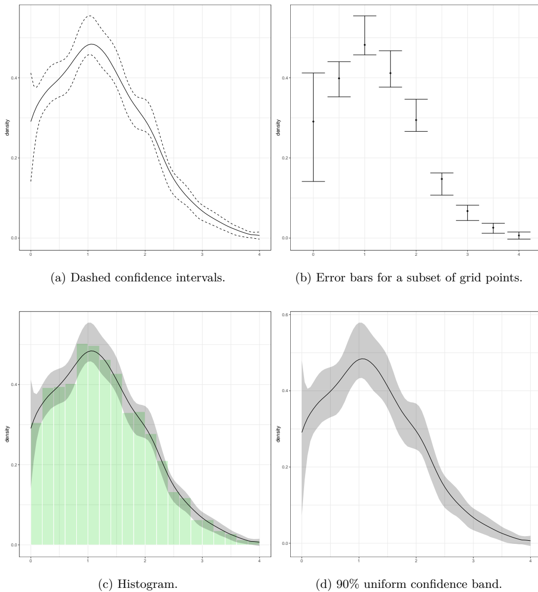
Figure 2: Density plots with different specifications.
