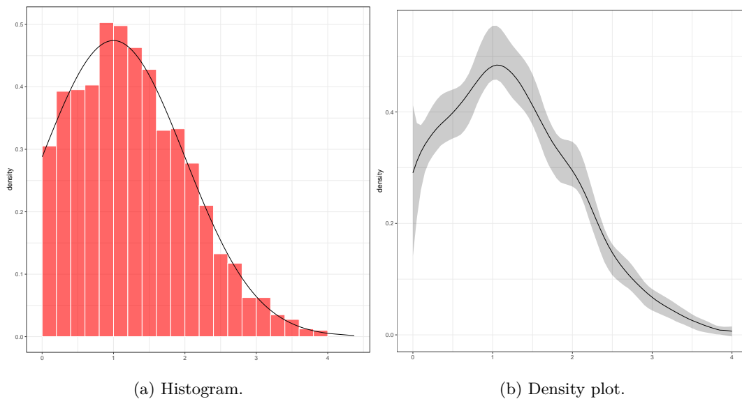
Figure 1: Histogram of the simulated data and the density plot.
