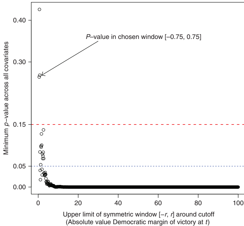
Figure 1: Window selector based on predetermined covariates.
